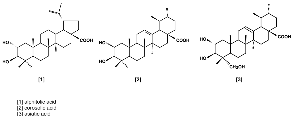
Figure 1. Alphitolic, corosolic, and asiatic acid structures.
